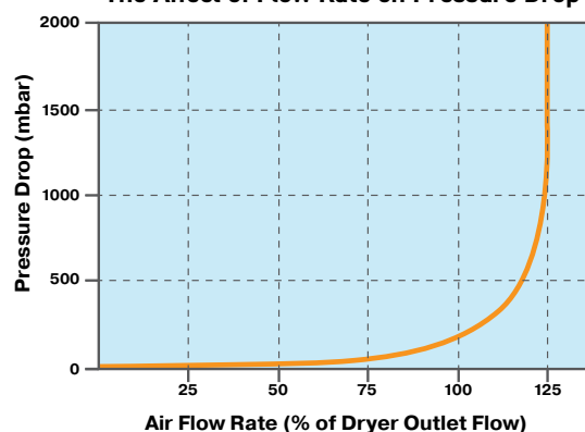
The Affect of Flow Rate on Pressure Drop
