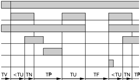
Process in case of pressure build-up failure, DS
