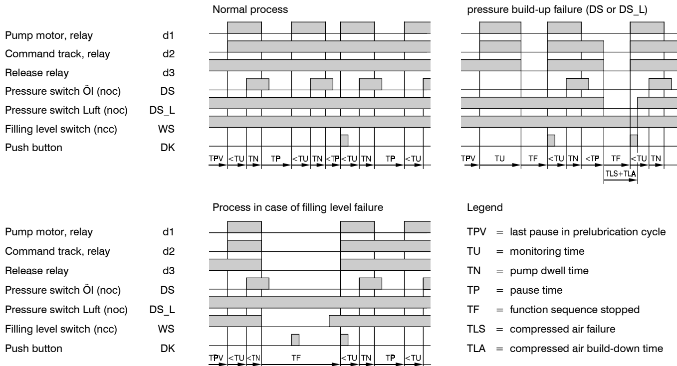
Figure 2 - 18. Pulse Diagram for IG54-20-S4
