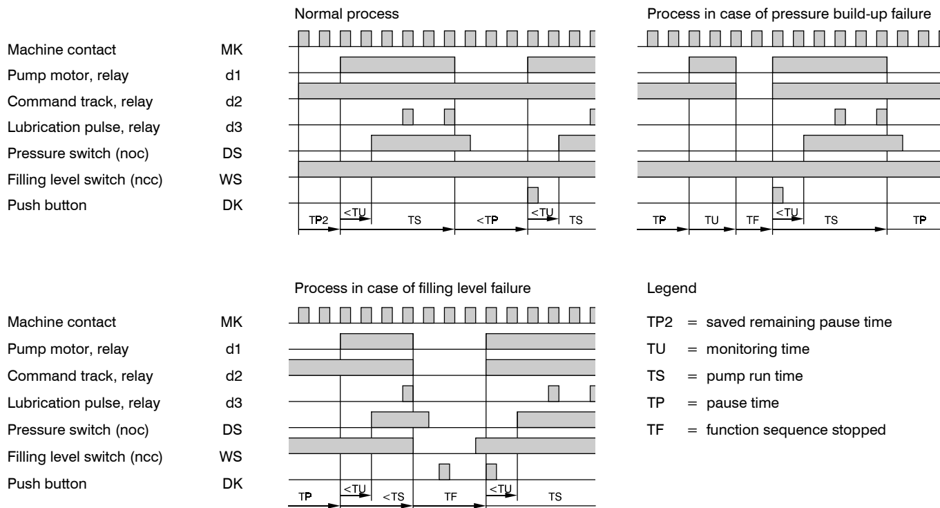
Figure 2 - 36. Pulse Diagram for IZ52-20
