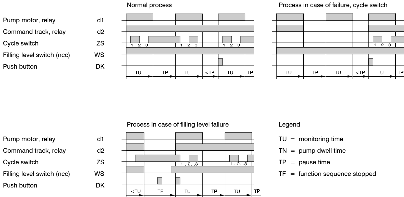
Figure 2 - 26. Pulse Diagram for IGZ51-20-S7
