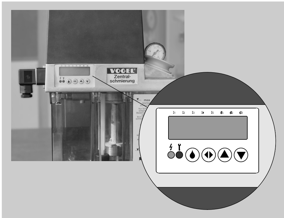
Figure 1 - 2. Operating Display of VOGEL Universal Controller for Industrial Lubrication System, Version I, Installed in Compact System
